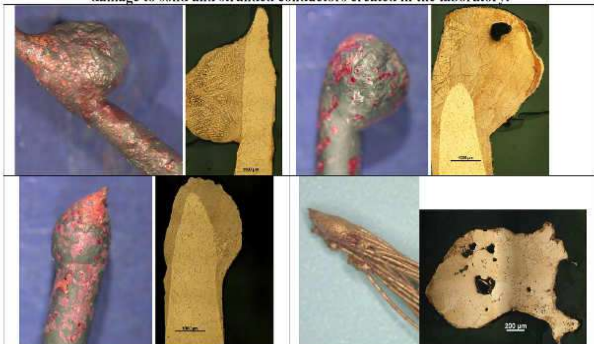
Figure 6 Stereomicroscope and optical micrographs of fire melting damage to solid and stranded conductors created in the laboratory.
