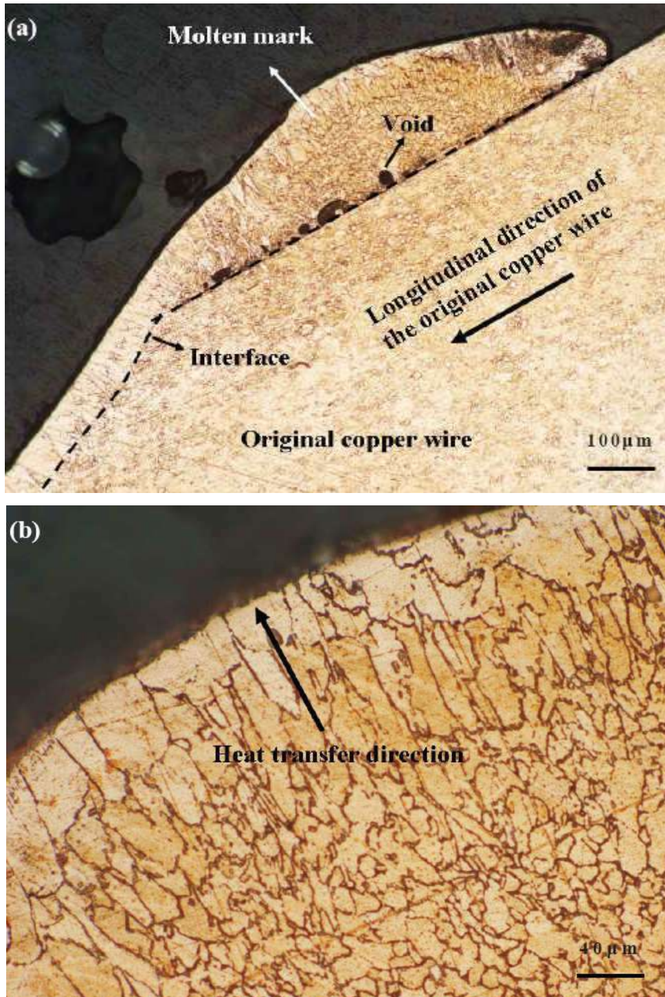
Esempi di osservazione al microscopio da: Microscopic Investigation of a Copper Molten Mark by Optical Microscopy (OM) and Atomic Force Microscopy (AFM) - GAO Ao, ZHAO Chang-zheng, DI Man, GAO Wei, ZHANG Ming, XIA Da-wei
